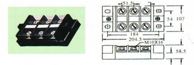
• ETB-400A
