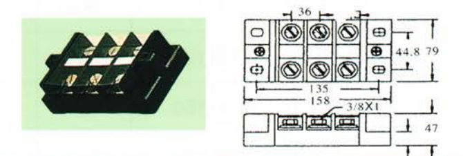
• ETB-400A
