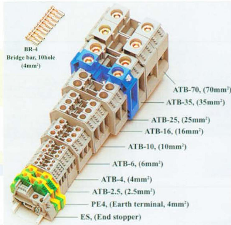
ATB 歐式端子盤 Screw Clamp Terminal Block Clip-On Mounting 2.5mm 2 ~70mm 2
