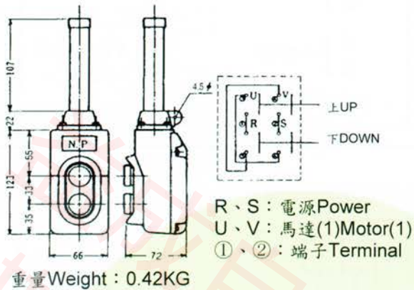
EOB-21 AC250V 15A 2點直接式2 Points Direct Input Type
