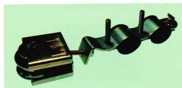
EH-D1雙孔銅滑輪 Double Hole Copper Trolley
