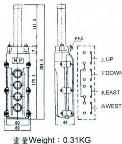
EOB-62 AC250V 5A 4點間接式 4 Points Indirect Input Type
