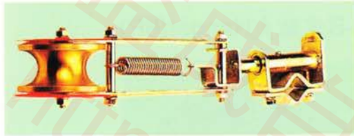
EH382集電架Collector Rack 加大銅輪型Large Copper Wheel Type 80mm
