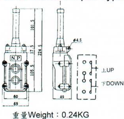
EOB-61 AC250V 5A 2點間接式 2 Points Indirect Input Type
