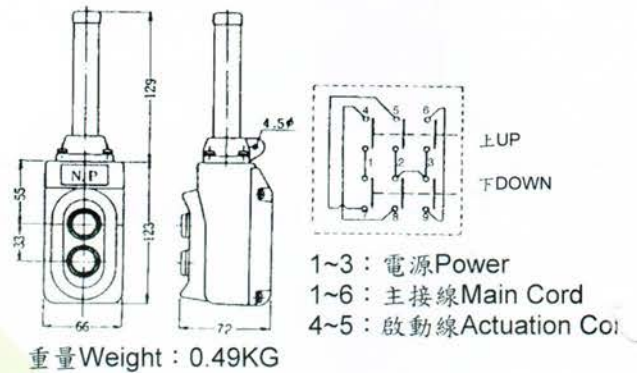
EOB-23 AC250V 15A 6點直接式6 Points Direct Input Type
