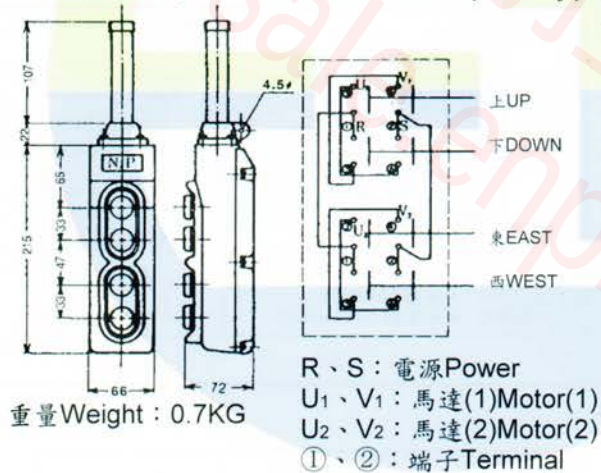
EOB-22 AC250V 15A 4點直接式4 Points Direct Input Type
