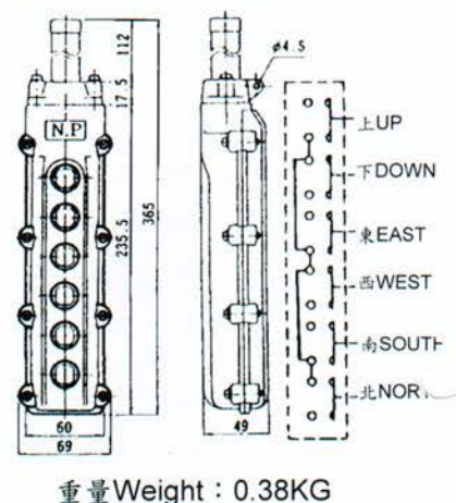
EOB-63 AC250V 5A 6點間接式 6 Points Indirect Input Type
