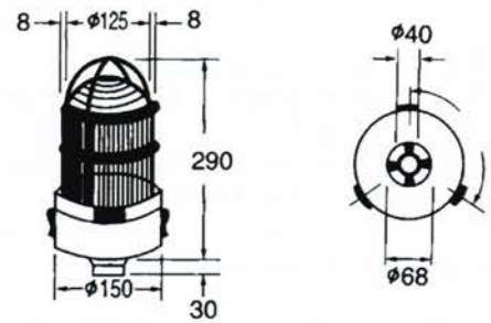
CT-15 大型高樓航空燈 Large Obstruction Light
