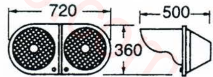
PC-C 橫式停車場紅綠燈 Horizontal Traffic Light
