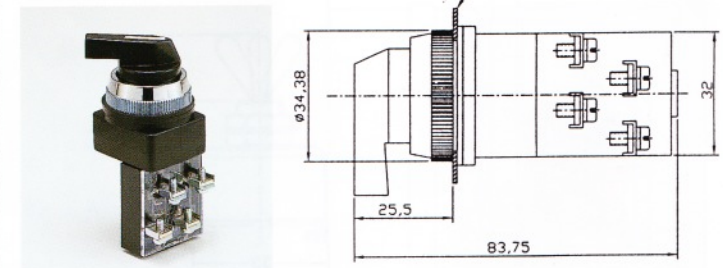
LSS3013, 3 position
