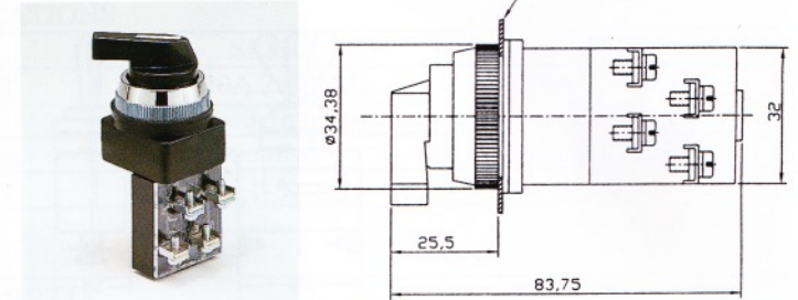
LSS3013, 3 position
