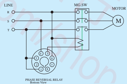
PHASE REVERSAL RELAY Bottom View
