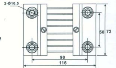
(437)CSH-10A-50A/50mv (438)CSH-60A-150A/50mv
