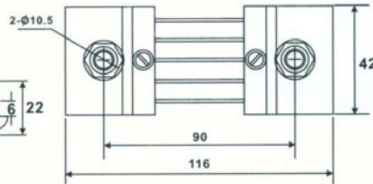
CSH3000A/50mv CSH4000A/50mv
