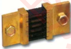
(443)CSH-600A/50mv
