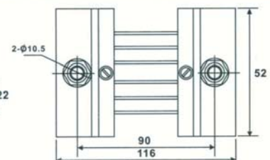
CSH5000A/50mv
