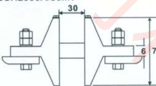
CSH1500A/50mv CSH2000A/50mv
