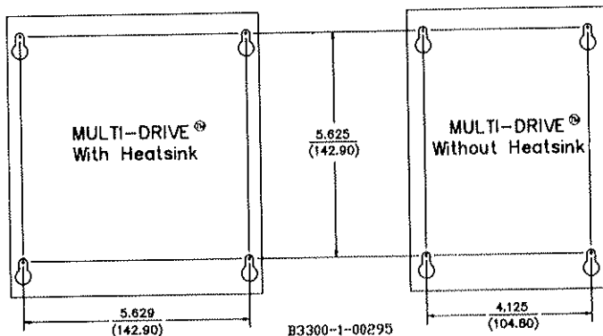
FIG. 3 MOUNTING DIMENSIONS (INCHES, MM)
