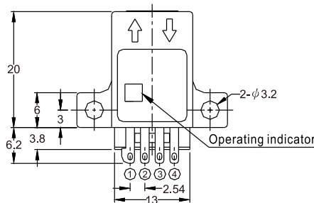
PNP Type
