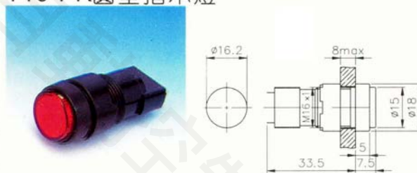
T16-PR圓型指示燈
