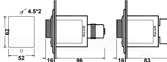
INSERT HOLE SH2-Y□ + US-08 SH2-Y□ + P3G-08
