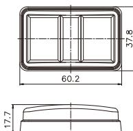
TN2-BTW (TN2-BT/IT用) 防水套
