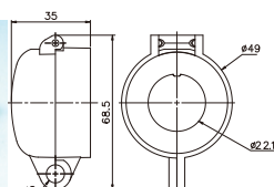
TN2-EAS(小型連鎖式護座無印字) TN2-EBS(小型連鎖式護座)
